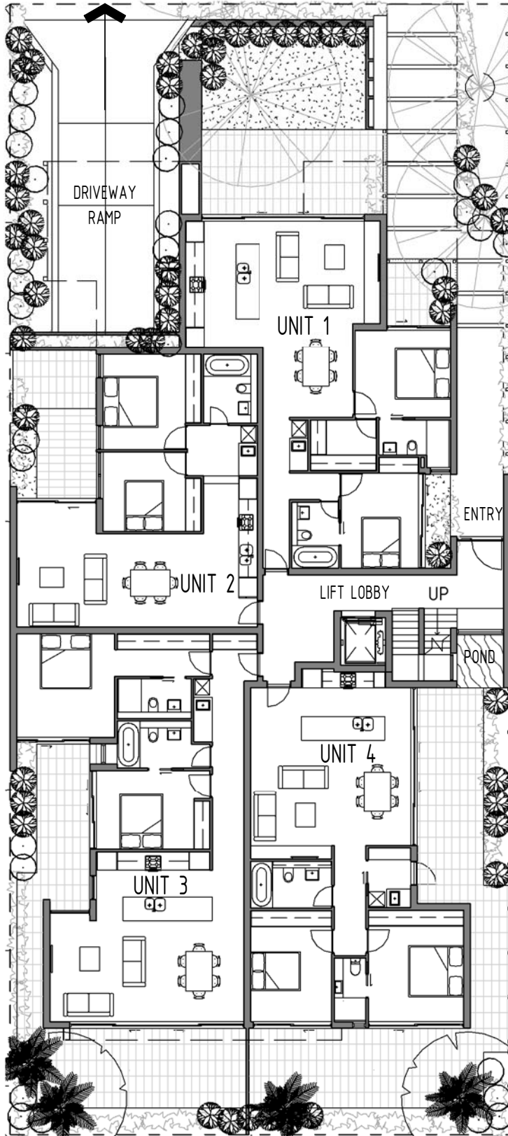
ground floor
